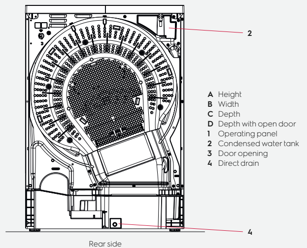
Rear side
