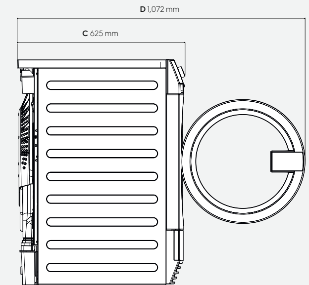
Right side
